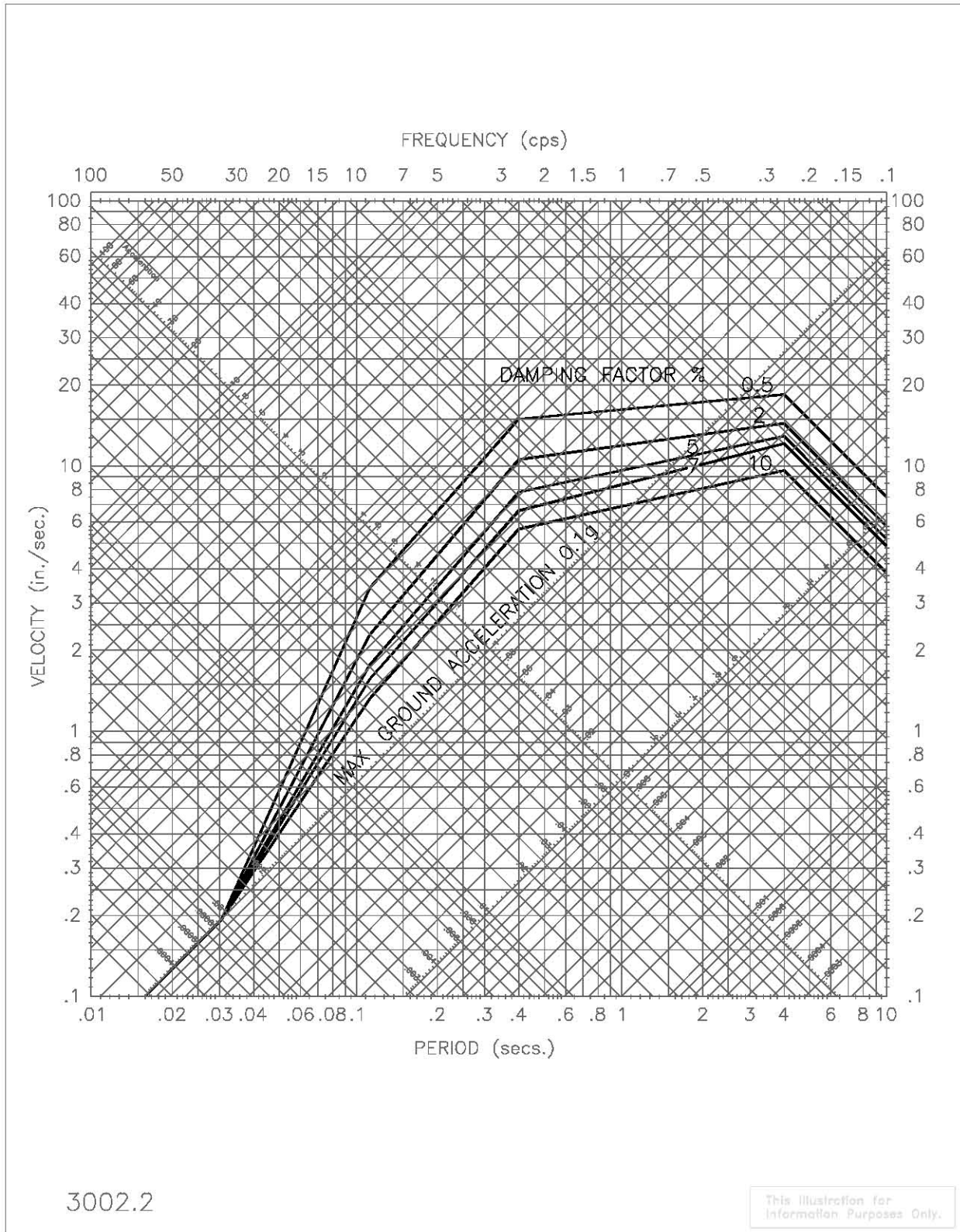
Figure 3.2-2, Horizontal Design Response Spectra
