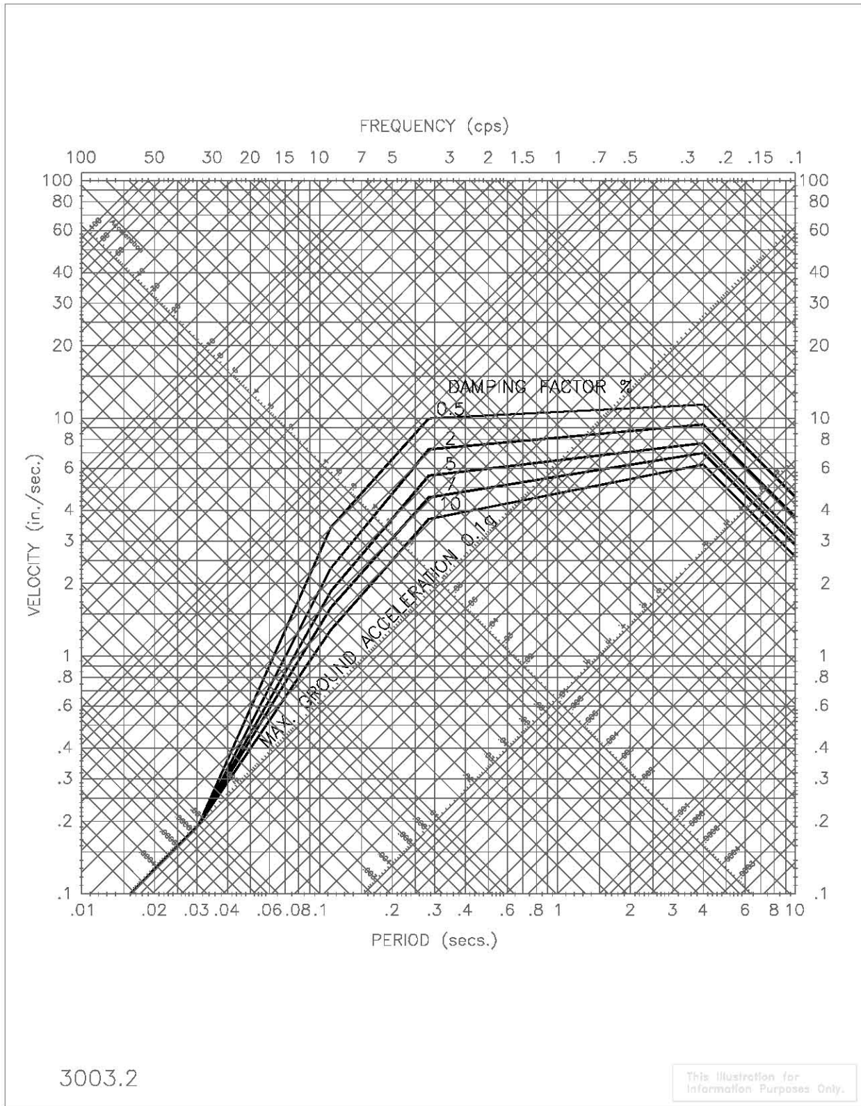
Figure 3.2-3, Vertical Design Response Spectra
